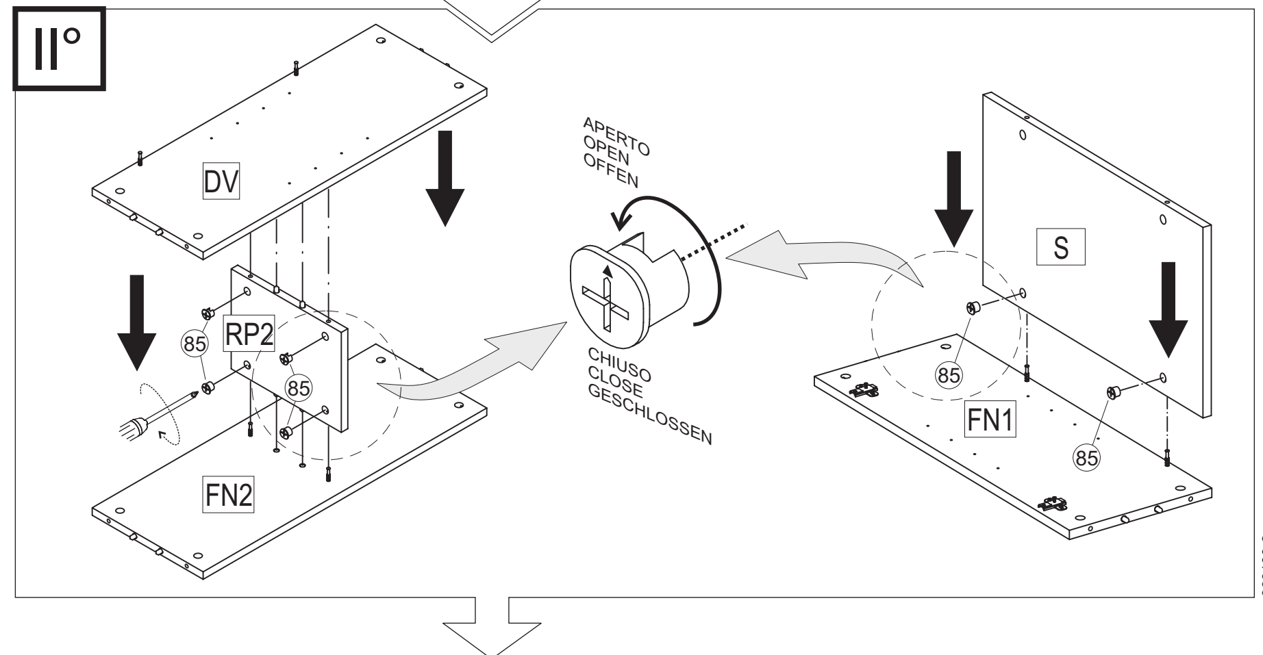
CAYMAN 60 623x343x730
