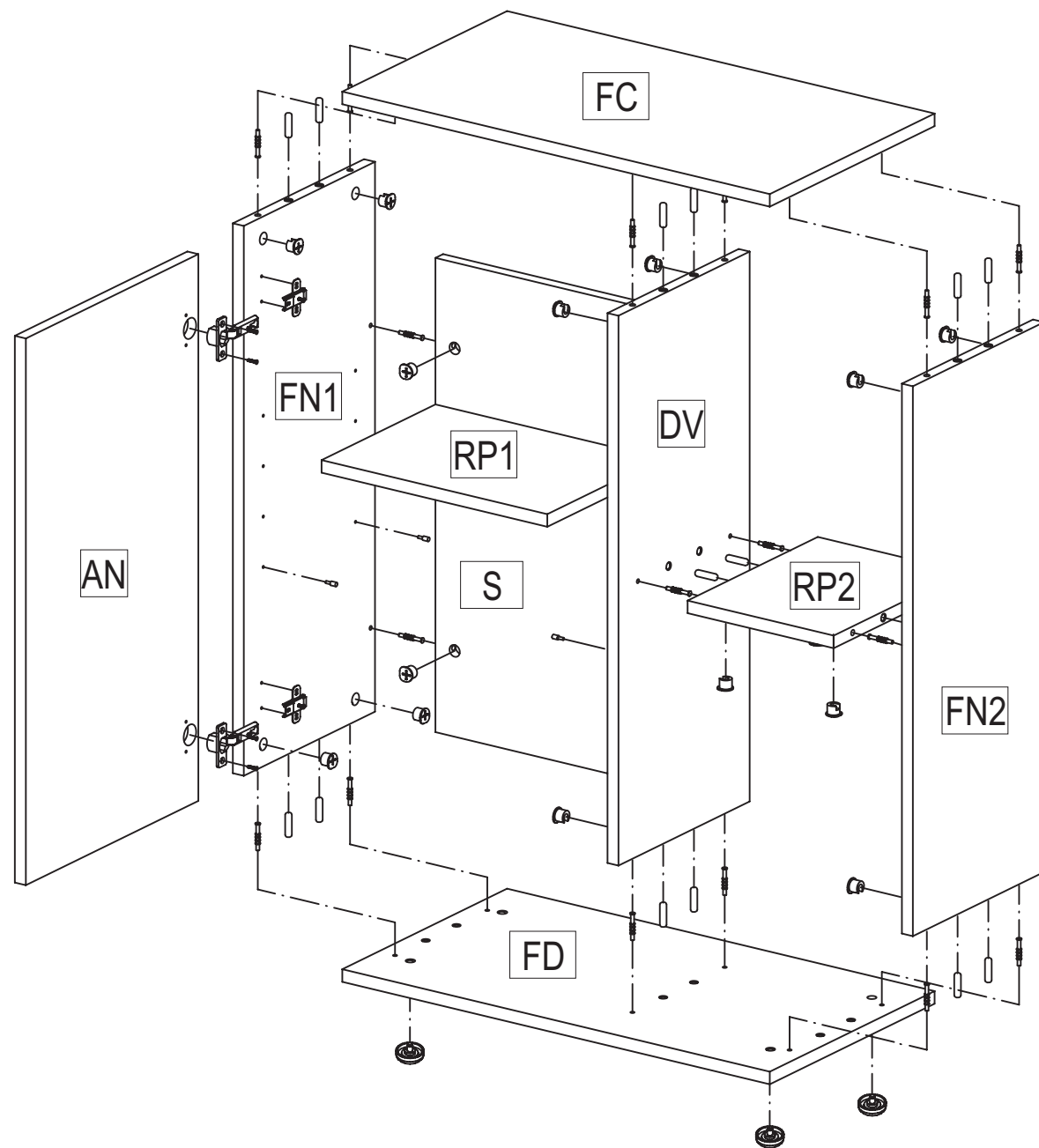
CAYMAN 60 623x343x730
